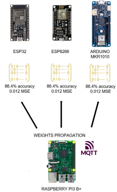
Fig. 6. Federated learning architecture - Weights propagation.
