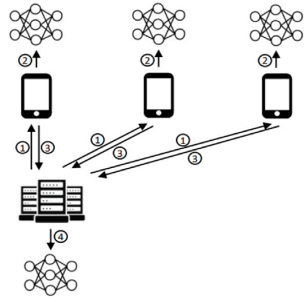
Fig. 3. Aggregation steps of the Federated Averaging (FedAvg) algorithm.
