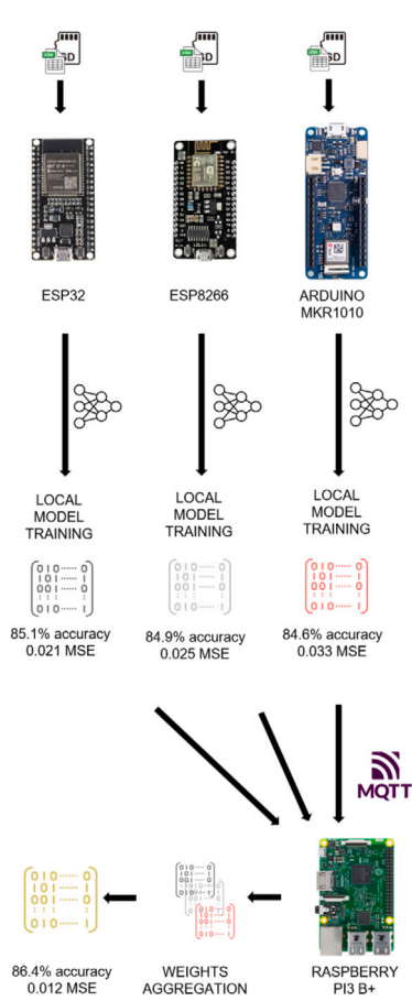
Fig. 5. Federated learning architecture - Training and weights aggregation.
